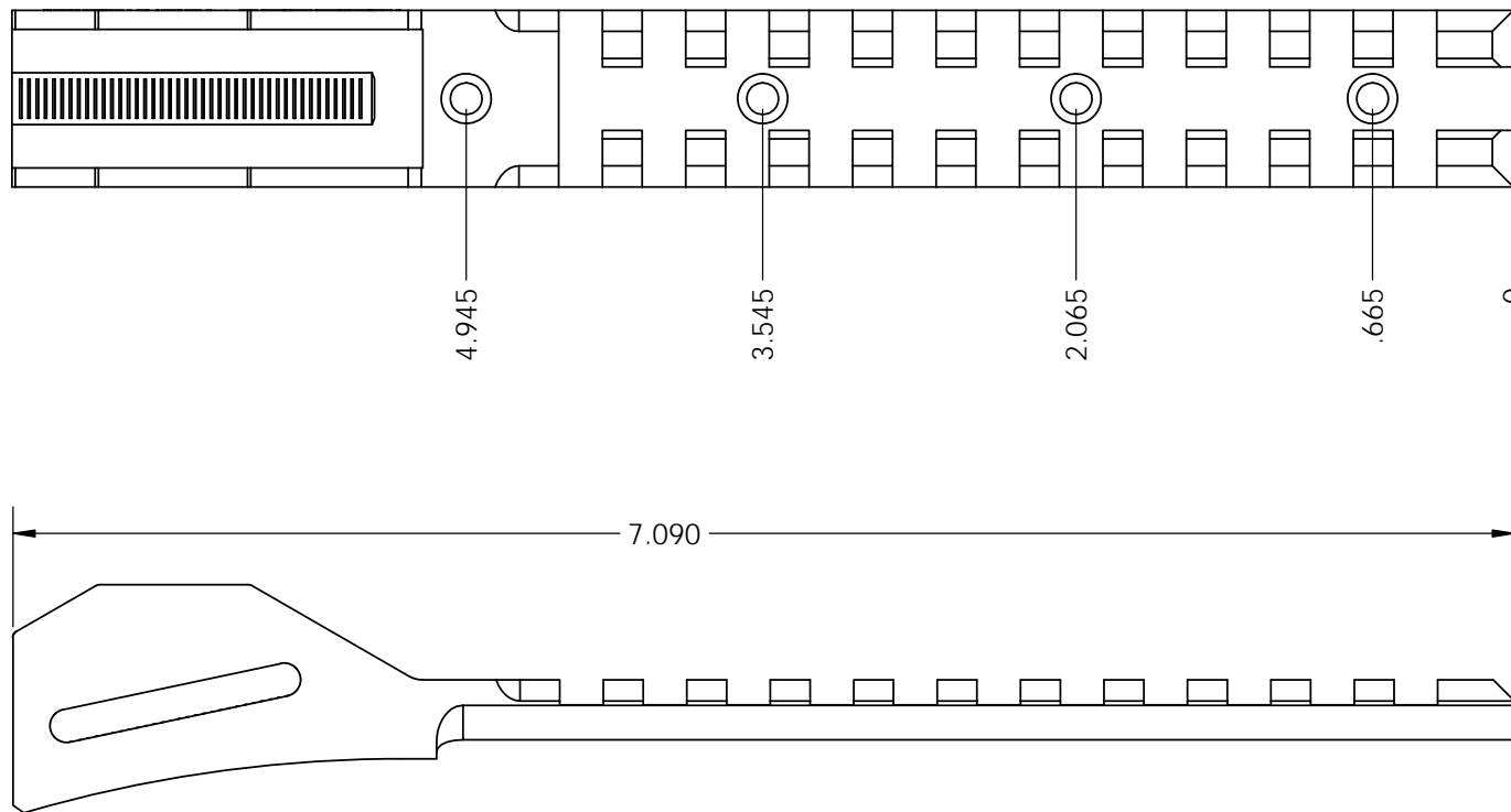
Hole pattern for standard 870 rail (scale 1:1)
